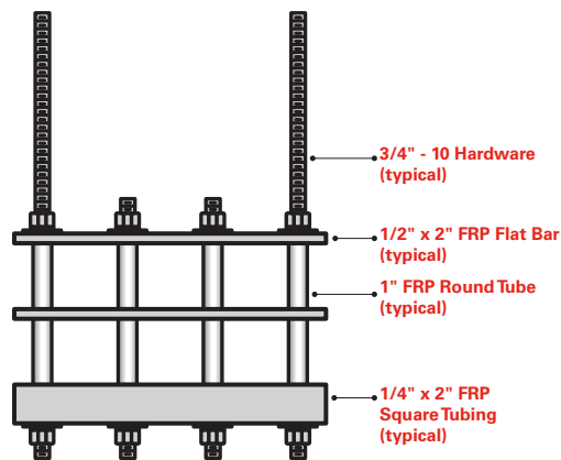
Intermediate Hanger / Flat Bar-Square Tube Bottom
