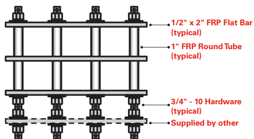
Diaphragm Hanger
