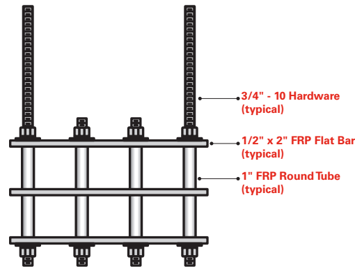
Standard Intermediate Hanger
