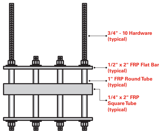
Intermediate Hanger / Flat Bar-Square Tubing-Flat
