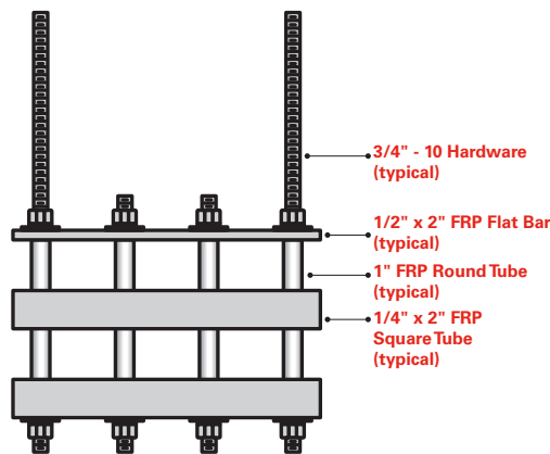
Intermediate Hanger / Flat Bar-Square Tubing
