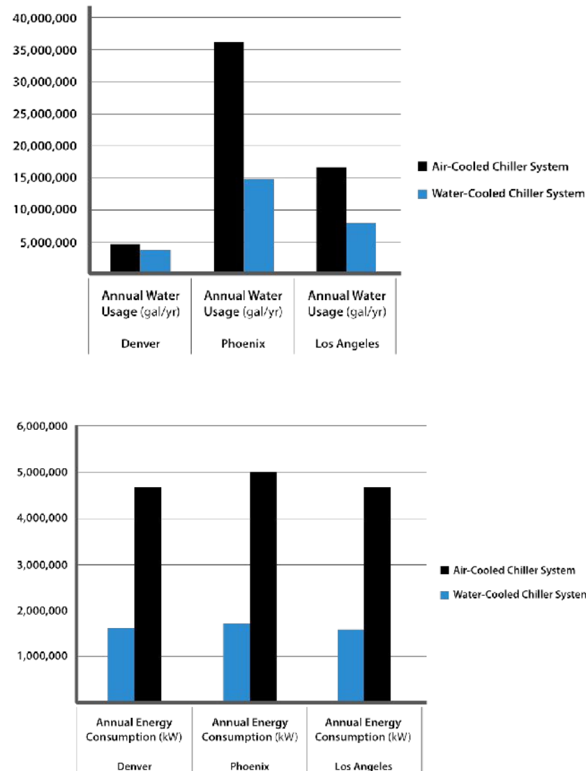
Figure 1 – Comparison of water and energy use in air-cooled and water-cooled chiller systems Source: Data Center Water Usage for Denver, Phoenix and Los Angeles: A Look at the big picture, by Tim Chiddix, PE, ATD and Brook Zion, PE, ATD
