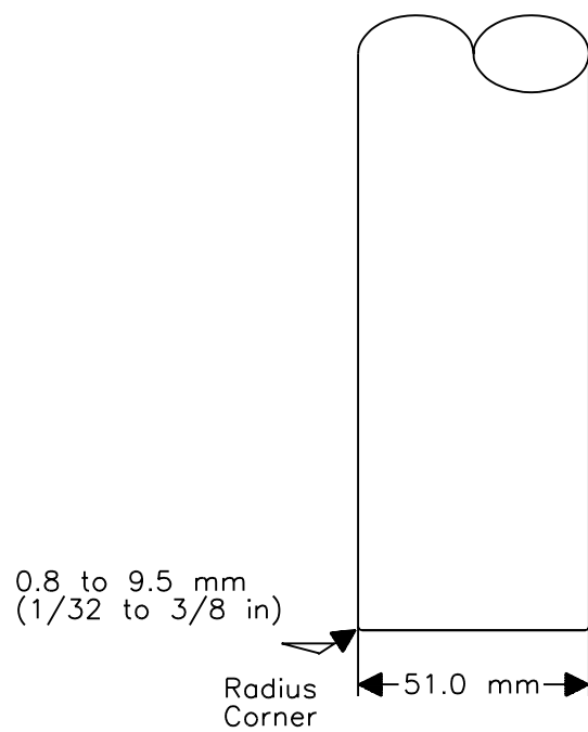
Figure 4 – Impact – tup geometry (See Clause 5.4.3)
